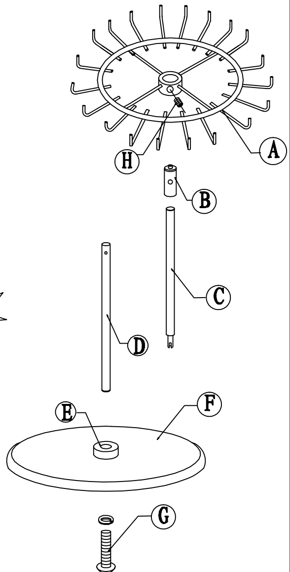
ASSEMBLY EXPLODED VIEW
